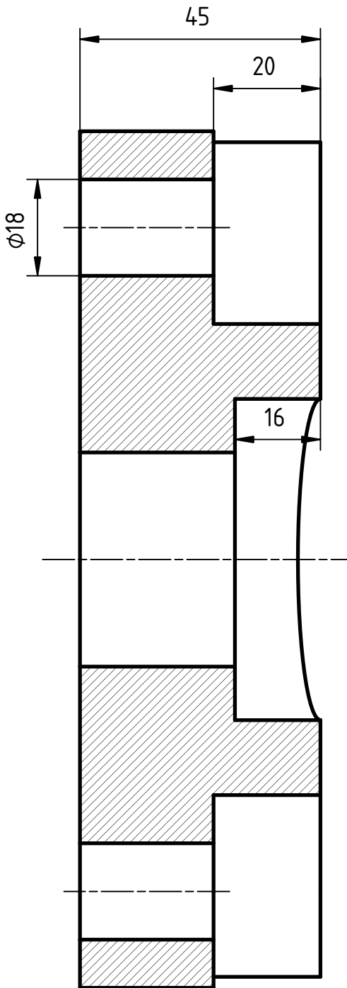
Section AA
